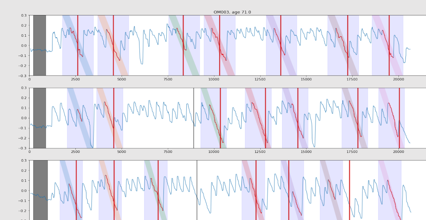
Fig3: The eye movement signals from the EyeGrip test for 3 speed conditions for one of the older subjects
