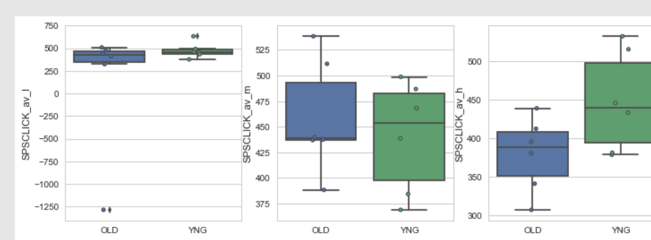
Fig10: The latency between the click event and the beginning of the target-SP
