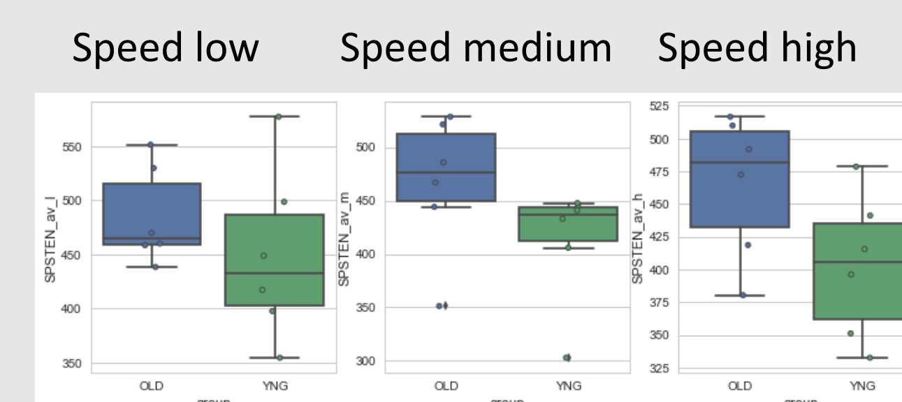
Fig5: The latency between the beginning of the SP on the target (target-SP) and the target enter
